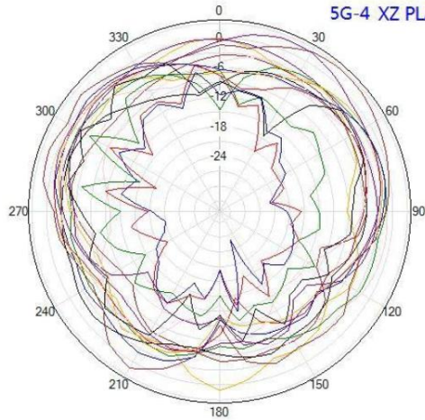
5G-4 XZ PLANE
