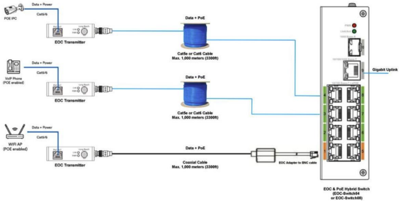
Figure 1-1 Typical application
