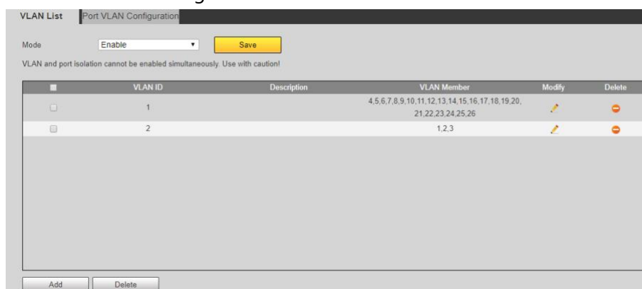
Figure 4-11 Enable VLAN
