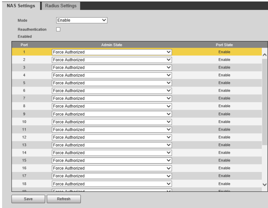
Figure 4-29 Configure NAS
