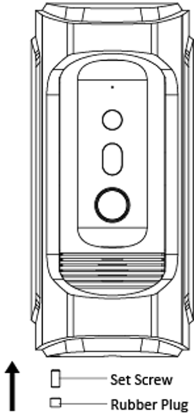
Figure 3-6 Secure the Doorbell
