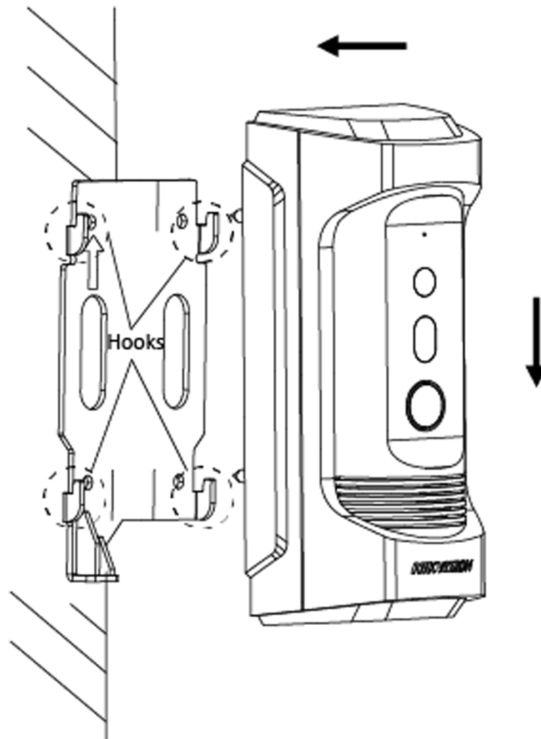
Figure 3-5 Hook the Doorbell to the Plate
