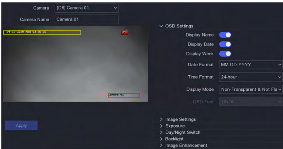
Figure 6-18 OSD
