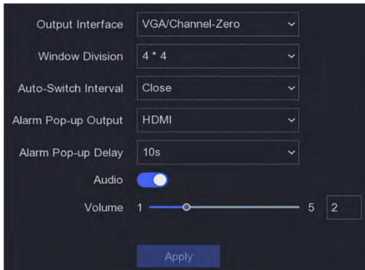
Figure 6-3 Live View-General
