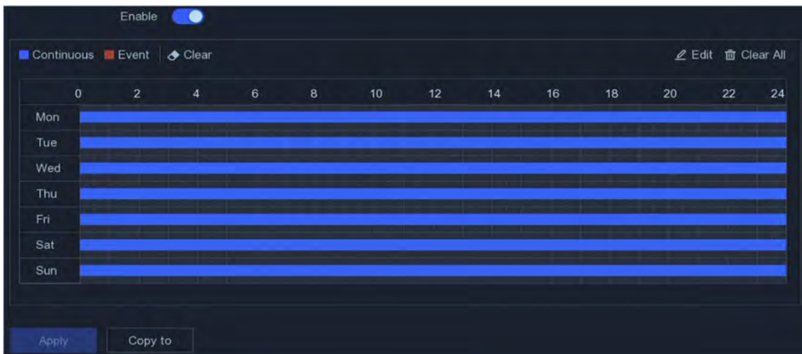
Figure 5-12 Recording Schedule
