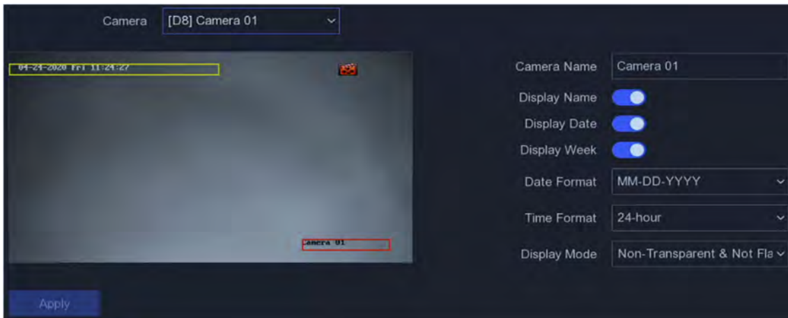
Figure 5-8 OSD
