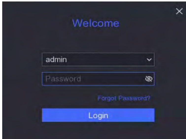
Figure 1-4 Login Interface
