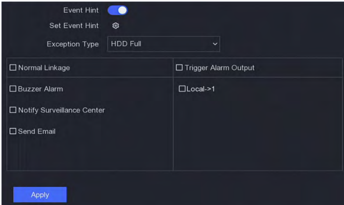
Figure 6-25 Exceptions
