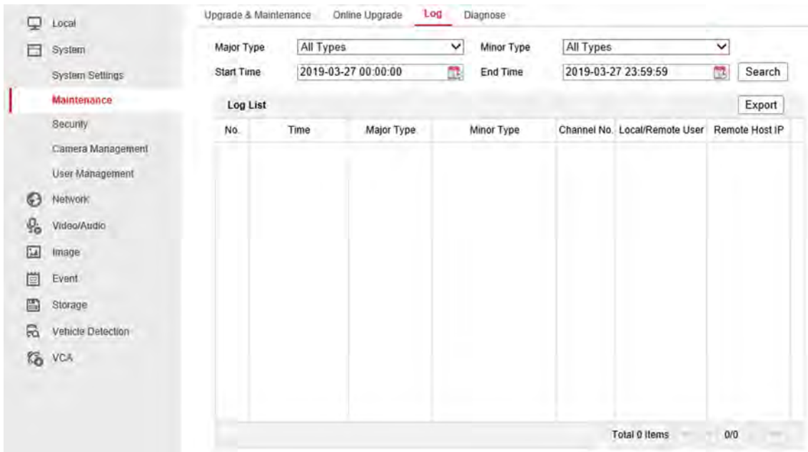
Figure 9-5 Log
