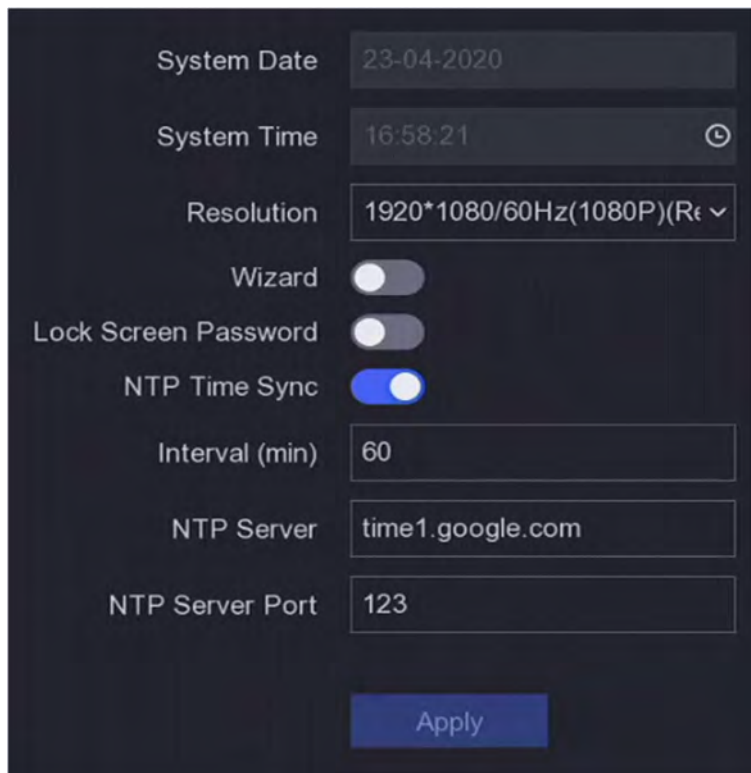
Figure 5-1 General Settings
