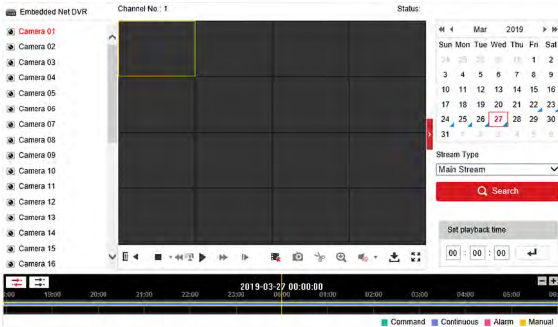
Figure 9-3 Playback
