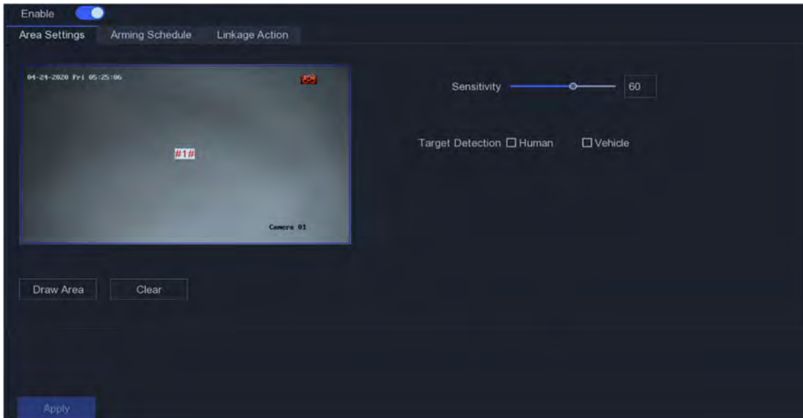
Figure 5-9 Motion Detection
