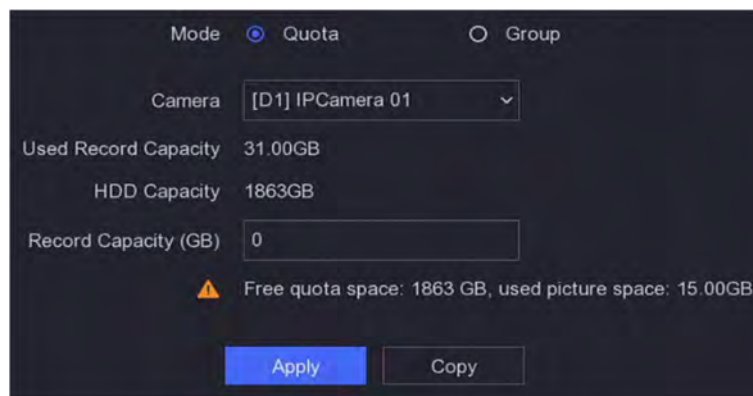
Figure 6-32 Quota
