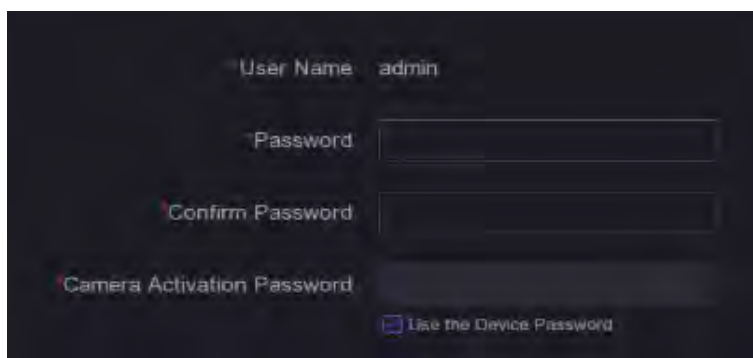
Figure 1-1 Activation
