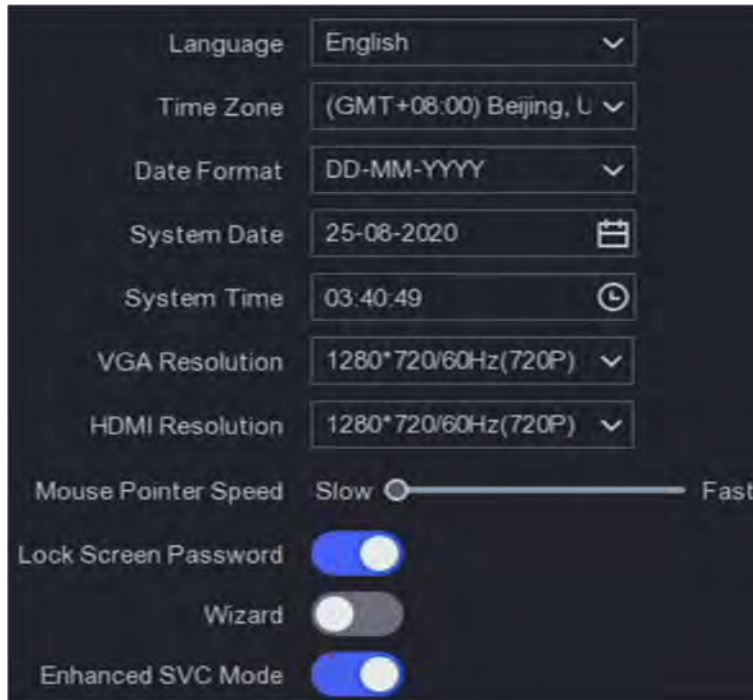
Figure 6-1 Basic Settings
