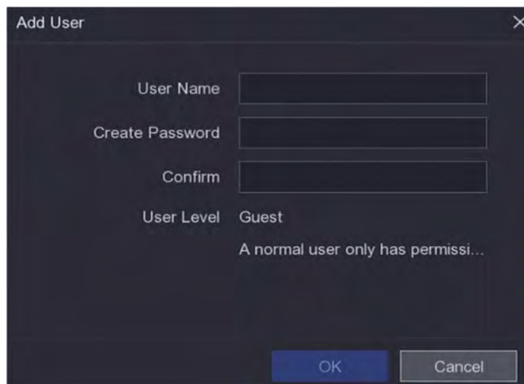
Figure 5-2 Add User
