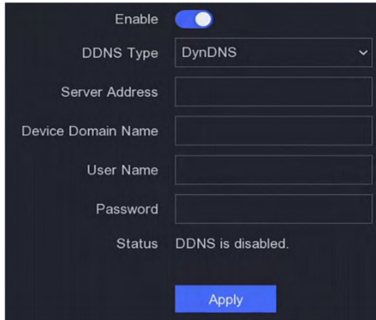
Figure 6-5 DDNS
