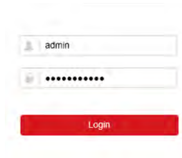
Figure 9-1 Login
