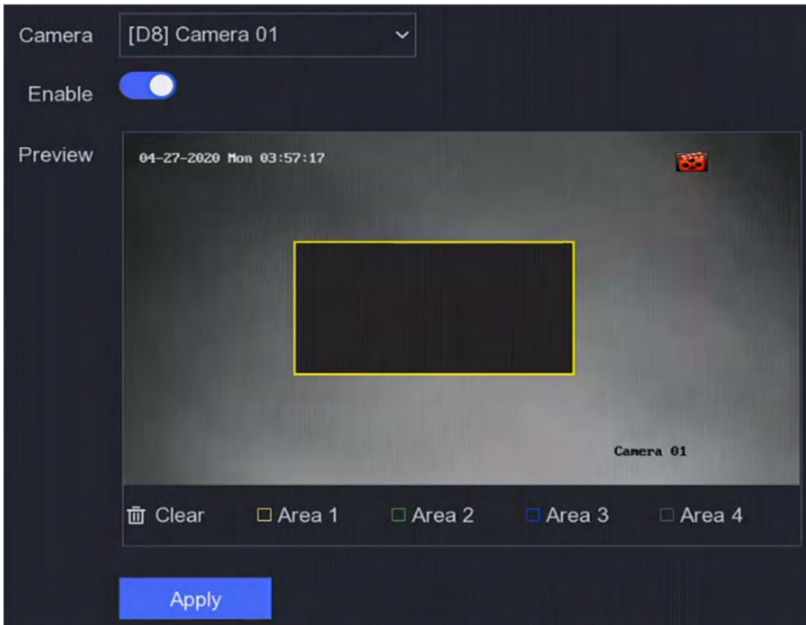
Figure 6-19 Privacy Mask
