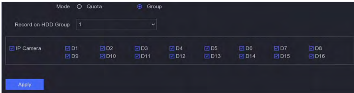
Figure 6-31 Group
