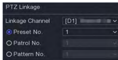
Figure 6-27 PTZ Linkage
