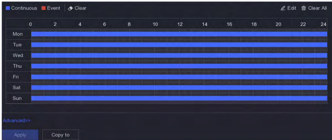
Figure 6-28 Recording Schedule
