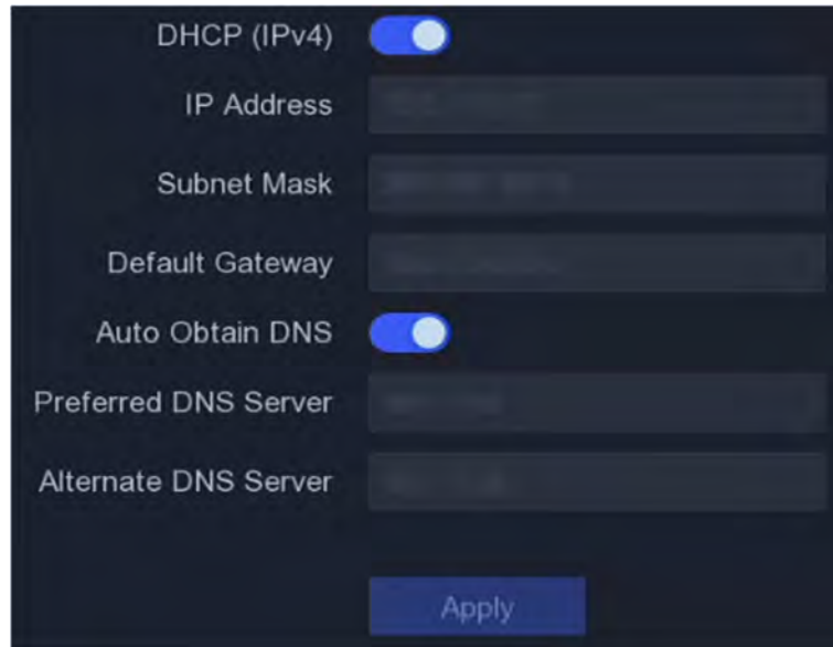
Figure 5-4 Network
