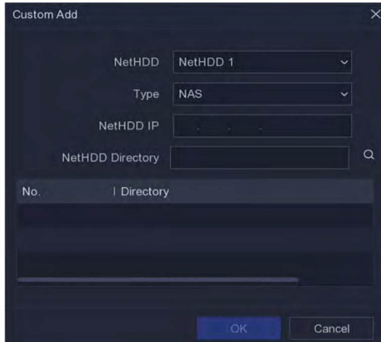
Figure 5-11 Add NetHDD
