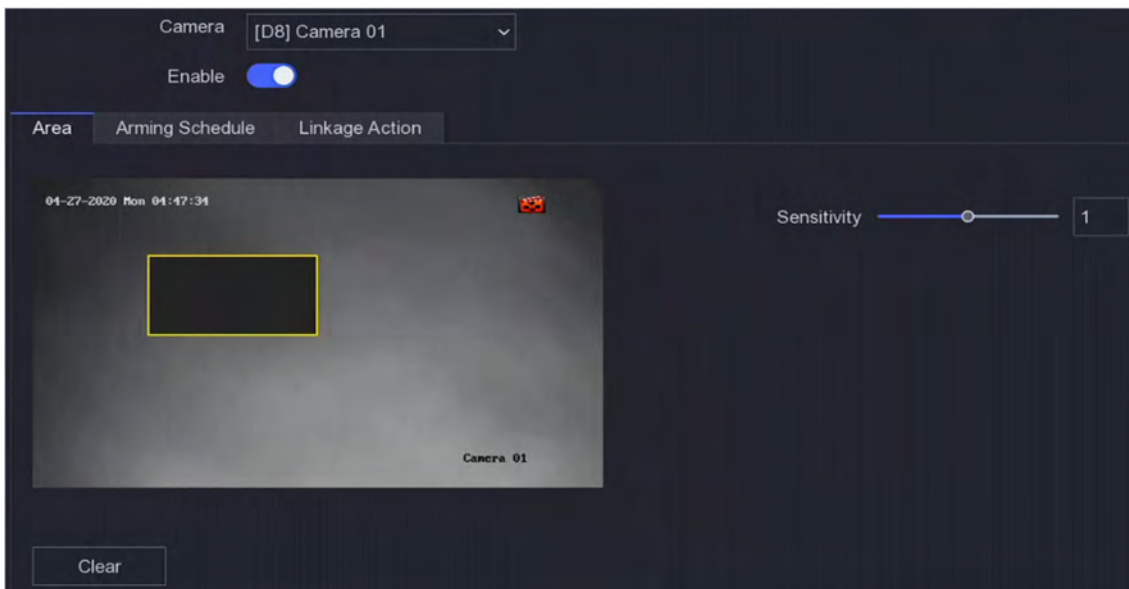
Figure 6-20 Video Tampering
