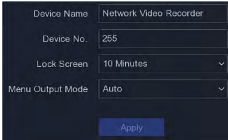
Figure 6-2 More Settings
